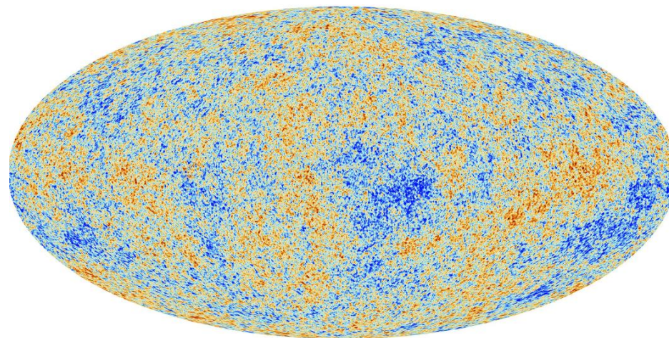
CMBR MAP (Planck)
